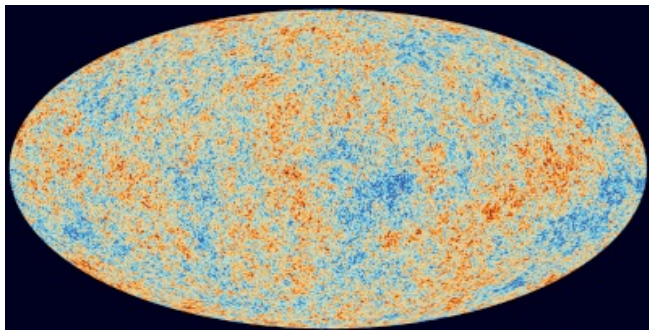
The Planck satellite's map of the cosmic microwave background.
